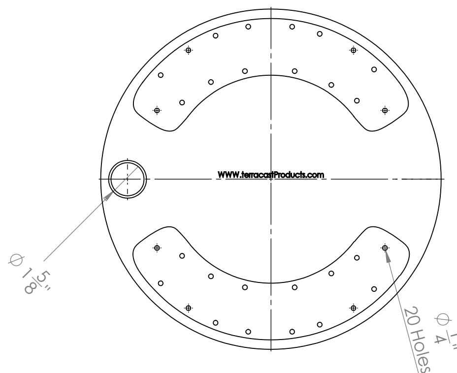
PLAN
