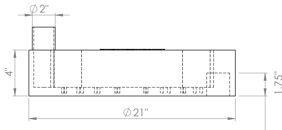
FRONT
